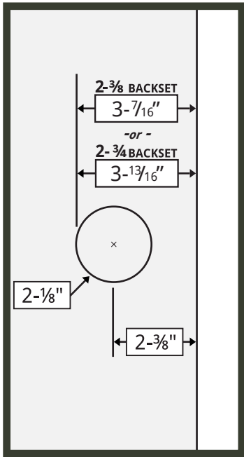
#100 • Standard Bore Prep
