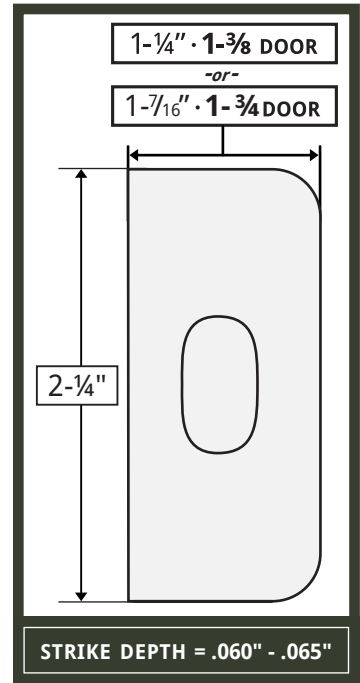
#300 • Standard Strike Prep
