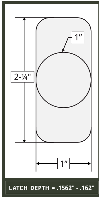
#200 • Standard Latch Prep
